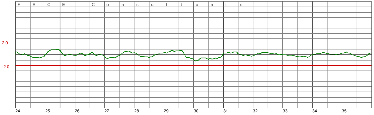
Right 2 Metre Graph
